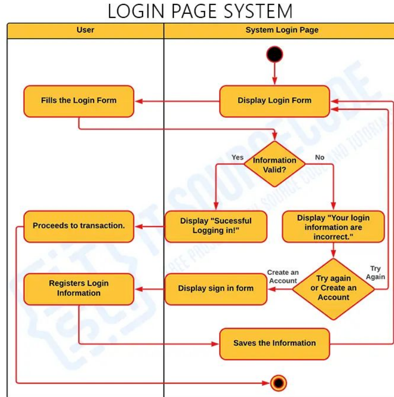
ACTIVITY DIAGRAM
